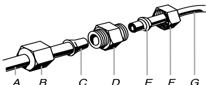
A. Refrigerator water tubing B. Nut (provided) C. Bulb D. Coupling (purchased) E. Ferrule (purchased) F. Nut (purchased) G. Household water line
